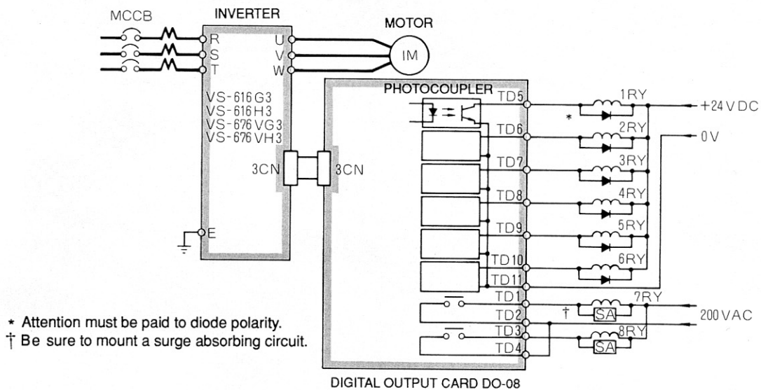
Fig. 2 Interconnection
